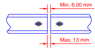
Front View of Termination Bar
